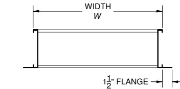
MODEL: 2625 FRAME: FLANGE FRAME FLANGE-MOUNT (FM)
